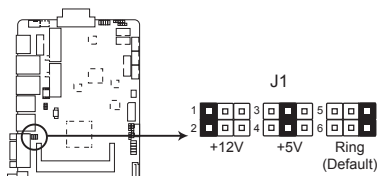
FAY-002 COM2 Ring/+5V/+12V Selection
