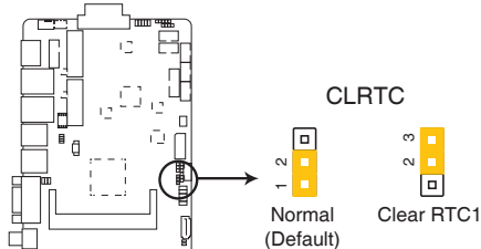
FAY-002 Clear RTC RAM
