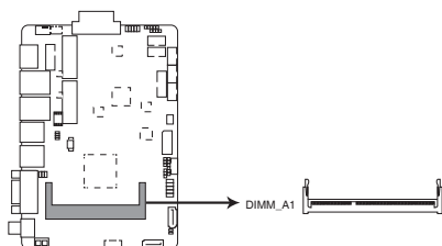
FAY-002 204-pin DDR3L DIMM socket
