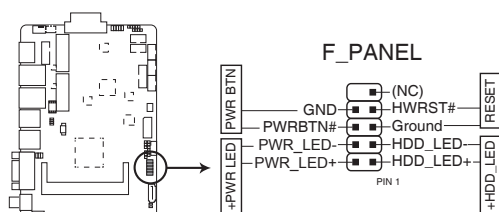
FAY-002 System panel connector
