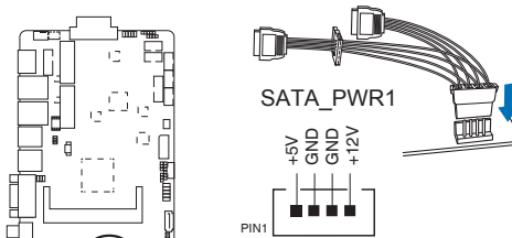
FAY-002 SATA POWER connector
