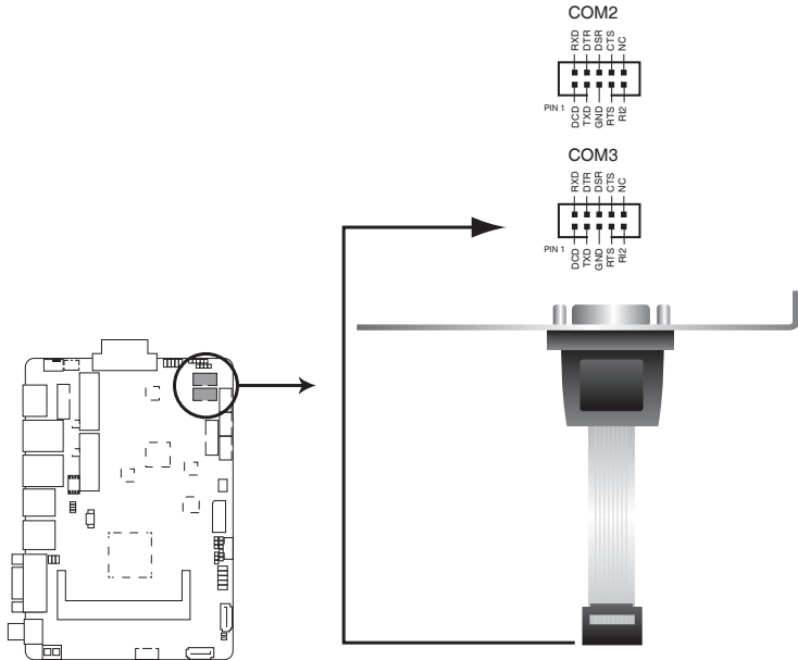
FAY-002 Serial port connectors
