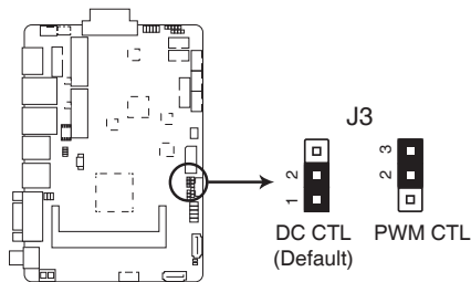
FAY-002 Mode Selection for Back Light Control of Inverter
