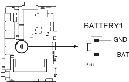
FAY-002 BATTERY connector
