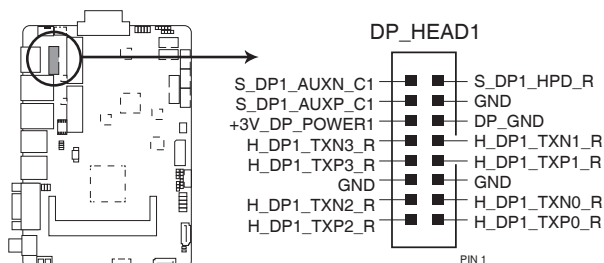
FAY-002 DP_HEAD connector
