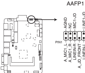
FAY-002 Front panel audio connector
