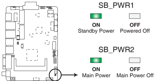
FAY-002 Onboard LEDs
