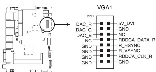
FAY-002 VGA connector
