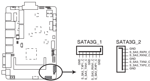
FAY-002 SATA 3.0Gb/s connectors
