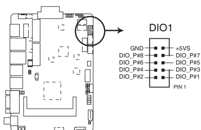
FAY-002 Digital I/O connector
