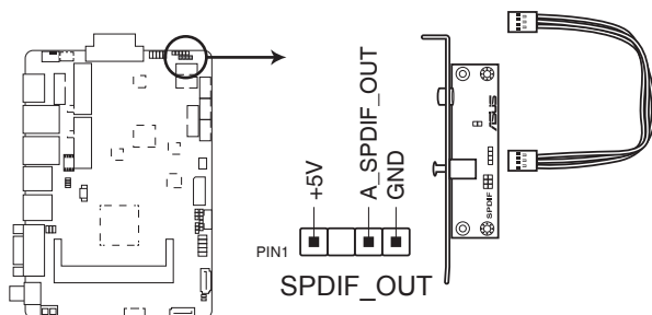
FAY-002 Digital audio connector
