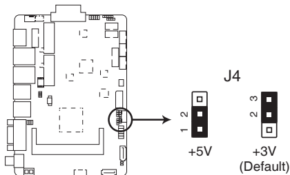
FAY-002 LVDS Panel Voltage Selection
