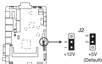
FAY-002 Inverter Voltage Selection
