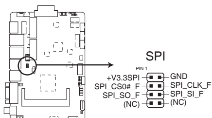
FAY-002 BIOS Programmable connector
