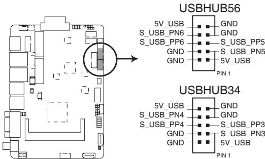
FAY-002 USB2.0 connectors
