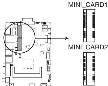
FAY-002 MINICARD connectors
